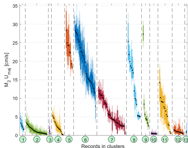
Fig. 4 Spatio-temporal variability of tidal currents, illustrated by the range of M_2 U_{\text{maj}} (from 30-day (light shading) and 90-day (solid colour) analysis, at 50 m depth) for each record in each cluster. The records within each cluster are sorted by average U_{\text{maj}} (black dots). For readability, horizontal plotting space was stretched for clusters with a smaller number of records (clusters #5 and #7–#13).
