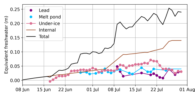
Figure 11. Summary of meltwater sinks (freshwater equivalent) from mid-June to late July. The total (black) includes estimated freshwater in leads (purple), melt ponds (cyan), under-ice (pink), and internal in the ice (brown).
