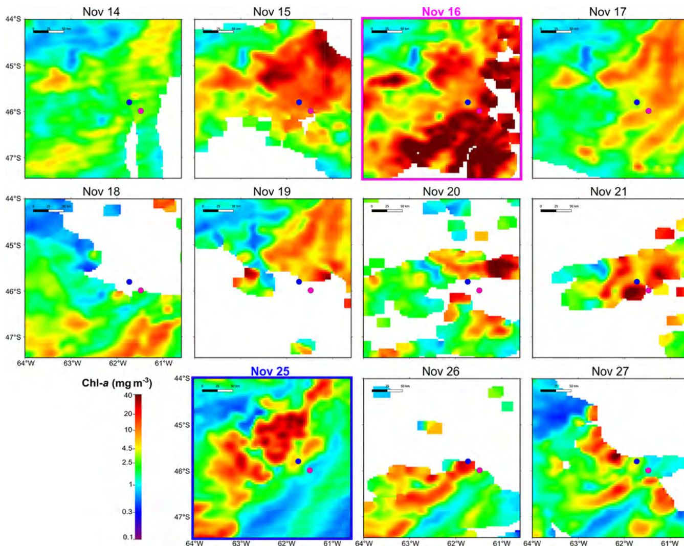
Figure 3. Daily satellite-derived surface chlorophyll a in the area of the sampling stations: GA01 (pink dot, sampled on 16 November 2021) and AA09 (blue dot, sampled on 25 November 2021).
