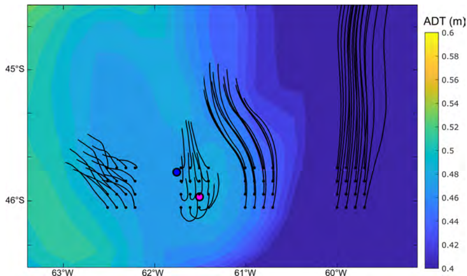
Figure D1. Background colours: absolute dynamic topography (m) averaged from 16 to 25 November. Black lines correspond to the advection of particles for the same period after release at the points indicated with a black dot on 16 November.
