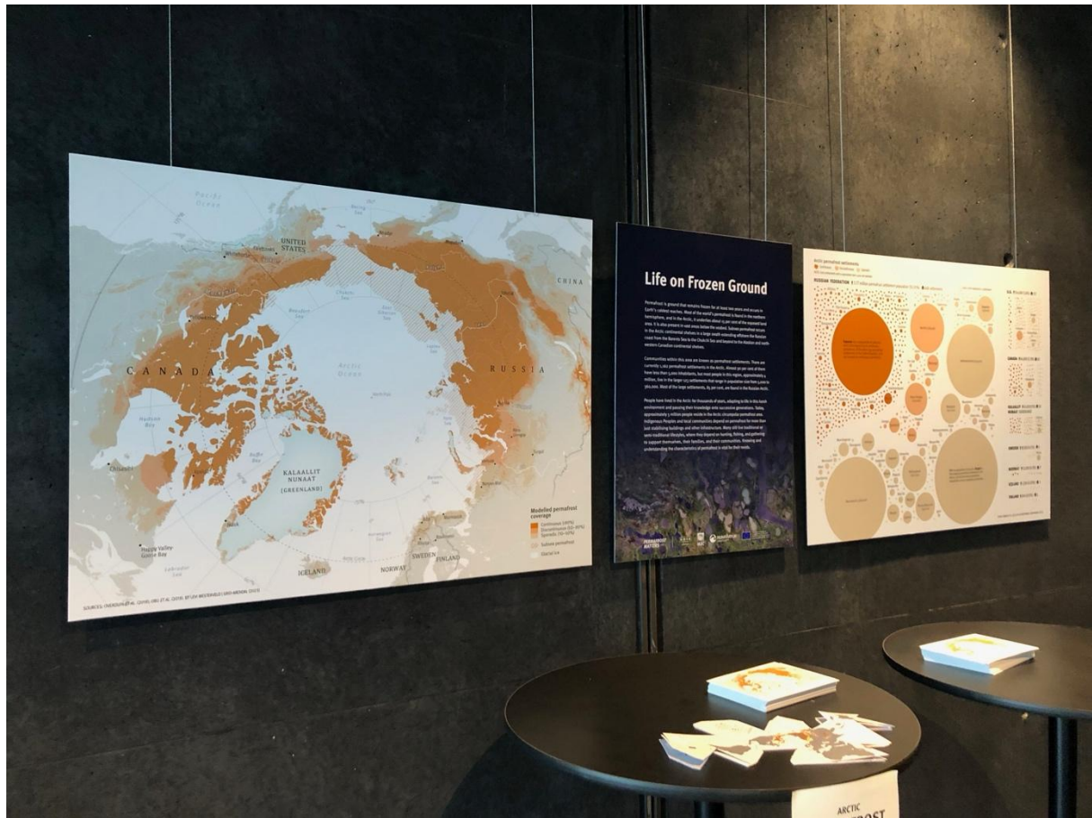
Figure: "Permafrost Matters" Exhibition panels at the launch of the Arctic Permafrost Atlas at the Arctic Circle Assembly in Reykjavik on 23 October 2023.
