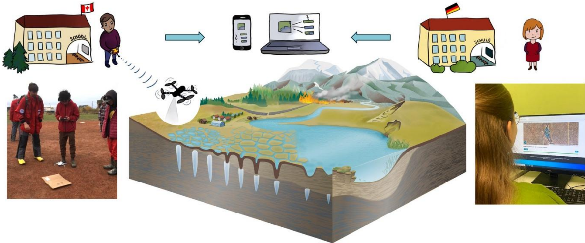
Figure: The concept of citizen scientists mapping permafrost polygons with drones (Canada) and digital mapping application (Germany).
