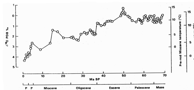
Figure 1.1 Temperature in Southern Ocean derived from oxygen isotope compositions ( \delta^{18}\text{O} ) of benthic foraminiferans. Water temperatures are calculated after making corrections for factors such as salinity and ice caps. The modern temperature scale is applicable to present day oceans, the Tertiary temperature scale to samples older than about 15 Ma (redrawn from Clarke 1983).
