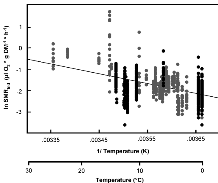
Figure 4.5 Fitted Arrhenius model of the relationship between mass-specific metabolic rates and temperature of 8 scallop populations (Black dots: own measurements; A. opercularis : McLusky 1973, Heilmayer et al. 2004; A. irradians irradians : Bricelj et al. 1987; A. irradians concentricus : Lu et al. 1999; C. islandica : Vahl 1978, Vahl and Sundet 1985; M. yessoensis : Fuji and Hashizume 1974; Z. patagonica : Heilmayer et al. 2001). Regression line: \ln(\text{SMR}_{\text{ind}}) = 11.851 - 3792.147 \cdot 1/T ( N = 953 , r^2 = 0.275 )
