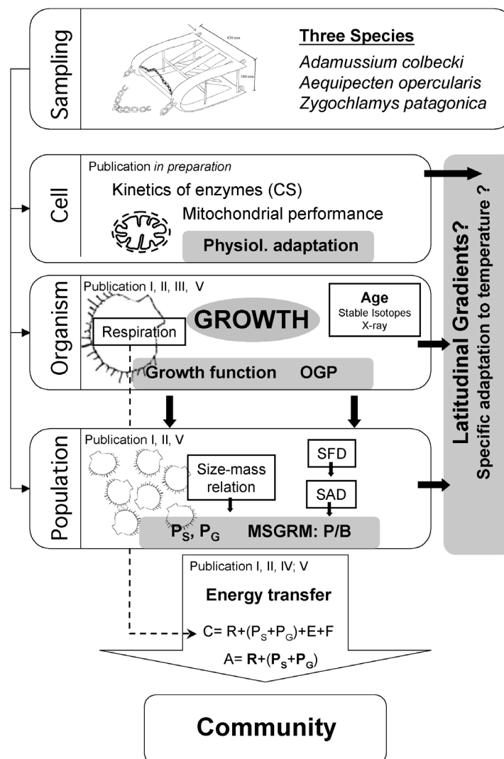
Figure 2.1 Flow chart demonstrating the hierarchical levels of life, which are possibly affected by temperature and the corresponding parameters investigated in this study. ( A : assimilation; C : consumption; CS : citrate synthase; E : excretion; F : faeces; MSGRM : mass-specific growth rate method; OGP : Overall growth performance; P G : gonad production; P s : somatic production; R : respiration; SAD : size-at-age data; SFD : size-frequency data)
