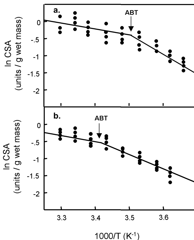
Figure 3.6 Temperature dependence of citrate synthase activity (CSA) in gill from a. A. colbecki and b. A. opercularis . Arrhenius-break-temperatures (ABT) calculated by the method of continuous two-phase regressions are indicated by arrows. ABT ( A.colbecki )=12.28° C; ABT( A. opercularis )= 19.41° C.
