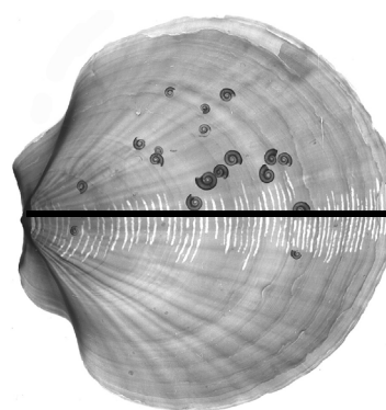
Figure 2.6 X-ray photograph of Adamussium colbecki showing annual growth marks (conspicuous rings of higher density) and sampling lines of shell carbonate for isotope analysis (white lines) along the height axis of the shell (black line).
