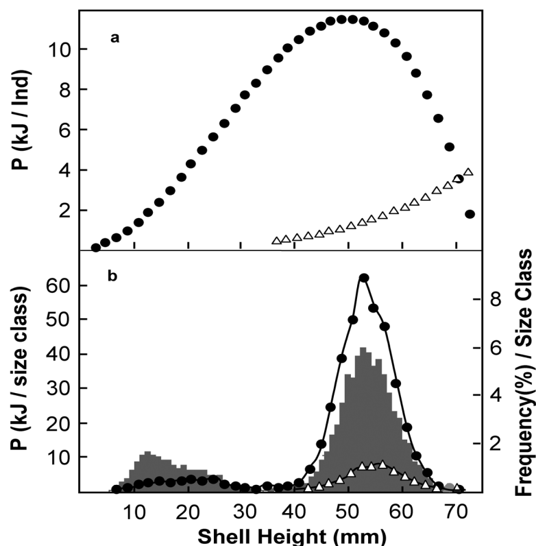
Figure 3.1 Zygochlamys patagonica . a. Individual production of somatic tissues (dots) and individual gonad production (triangle) for different size classes b. Size specific distribution of annual somatic tissues and gonad production at the population level, based on the pooled SFD of 2000.
